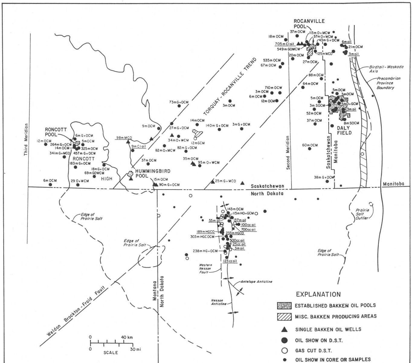
Figure 14: Diagram showing the relationship of structural features to oil shows and oil production within the study area. Major oilfields producing from the middle member of the Bakken Formation, oil shows from drill stem tests, cores or samples, and gas shows are indicated. Limit of the Prairie Formation salt is from Høltér (1969), Anderson and Swinehart (1979), and McCabe (1980).
