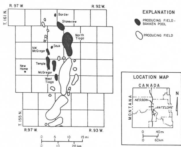
Figure 17: Map showing the distribution of producing oil fields along the northern Nesson anticline. Fields producing from the middle member of the Bakken Formation are indicated in black.
