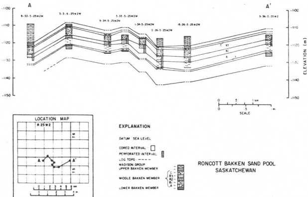
Figure 11: Structural cross-section showing the distribution of lithofacies units across Rencott field, Saskatchewan. Lithologies represented were described from core.
