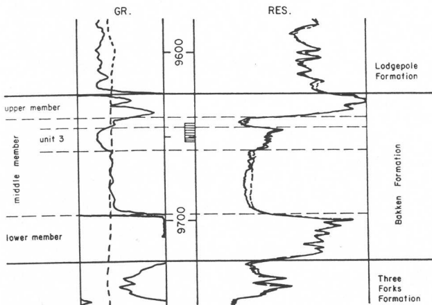
Figure 6: Typical log of the Bakken Formation in North Dakota. The three informal members of the formation are indicated. Unit 3 is the producing sandstone in the study area.
