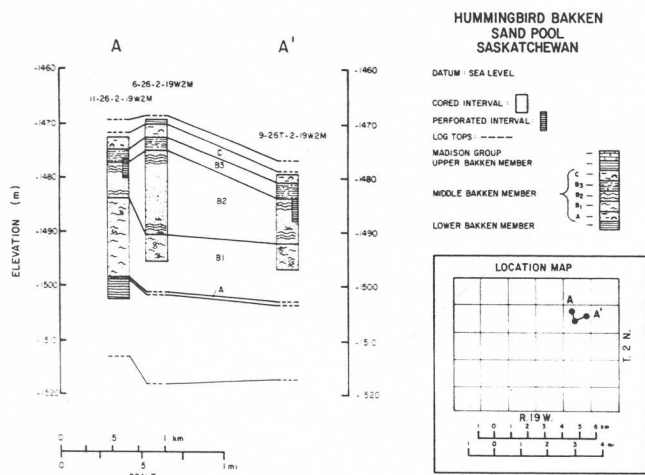
Figure 12: Structural cross-section showing the distribution of lithofacies units across Hummingbird field, Saskatchewan. Lithologies represented were described from core.
