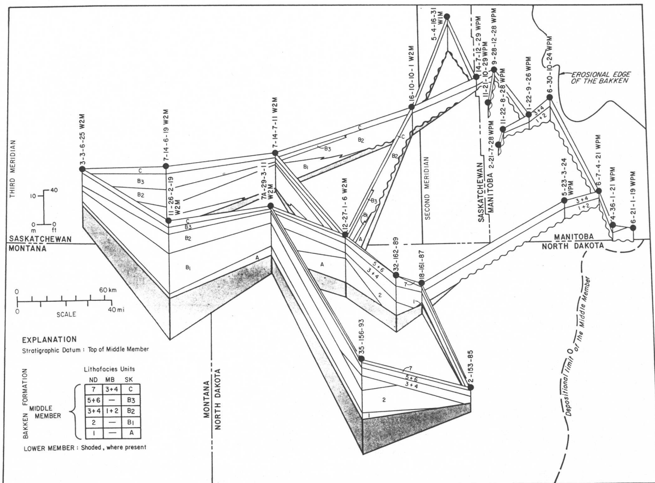
Figure 4: Regional fence diagram showing the distribution of the lithofacies of the middle member of the Bakken Formation. The lower member is shaded where present. Lithofacies units with their appropriate number or letter designation are shown.
