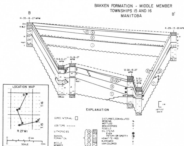
Figure 9: Fence diagram showing the distribution of the lithofacies units of the Middle Member of the Bakken Formation in Townships 15 and 16, Manitoba. Lithofacies represented are described from cores. Sedimentary features, as well as oil staining are indicated.
