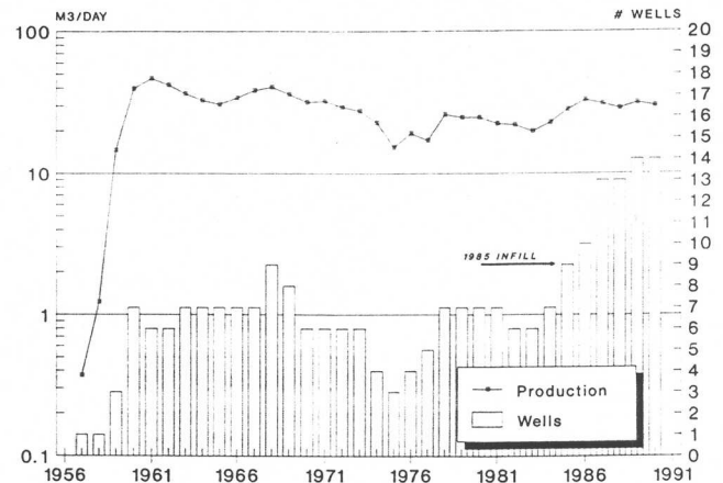
Figure 22: Average daily oil production by year for the Rocanville Bakken sand pool in Saskatchewan.
