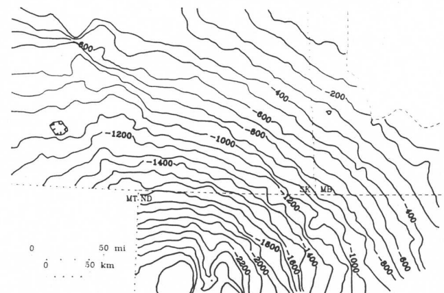
Figure 13: Structure map on the top of the Bakken Formation. Contour interval is 100 m (328 ft). Dashed line in northeastern Manitoba is the erosional limit of the Bakken Formation.
