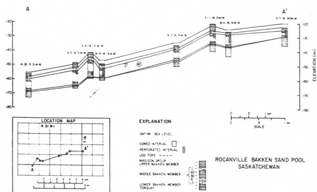
Figure 10: Structural cross-section showing the distribution of lithofacies units across Rocanville field, Saskatchewan. Lithologies represented were described from core.
