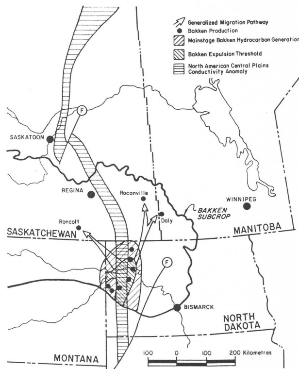
Figure 25: Diagram showing the area of mainstage hydrocarbon generation in the Bakken Formation. The area where the Bakken has exceeded its expulsion threshold is also indicated, as well as, the generalized migration pathway (from Osadetz et al. , 1991).
