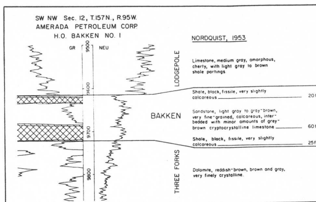
Figure 3: Type log for the Bakken Formation from Amerada Petroleum Corporation - H.O. Bakken #1 deep test. Lithologic description is from Nordquist (1953).
