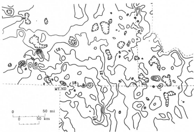
Figure 16: Isopach map of the middle member of the Bakken Formation for the study area. Contour interval is 3 m (10 ft). Dashed line in northeastern Manitoba is the erosional limit of the Bakken Formation.
