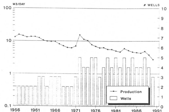
Figure 23: Average daily oil production by year for the Roncott Bakken sand pool in Saskatchewan.
