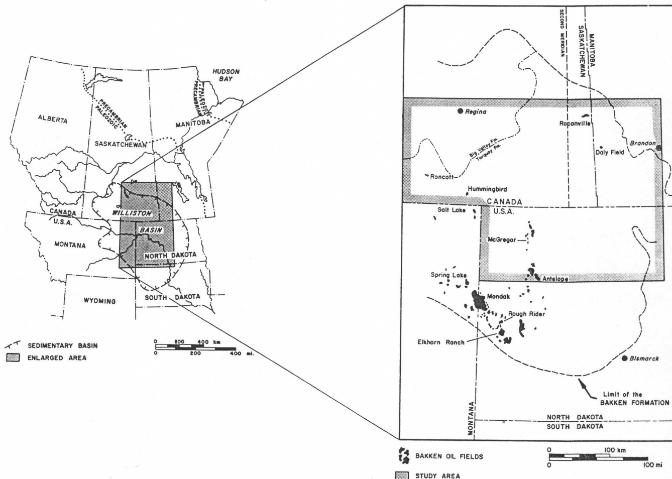
Figure 1: Index map showing the location of the study area within the Williston Basin. The approximate limit of the Bakken, Torquay, and Big Valley formations is indicated. Oil fields which are producing or have produced from the Bakken Formation are also shown.
