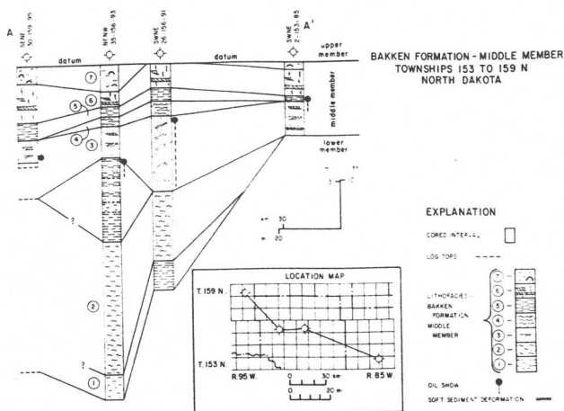
Figure 5: Fence diagram showing the correlation of lithofacies units of the middle member of the Bakken Formation from Townships 153 to 159 N, North Dakota. The lithofacies represented were described from cores. Oil shows are indicated over the interval where present.
