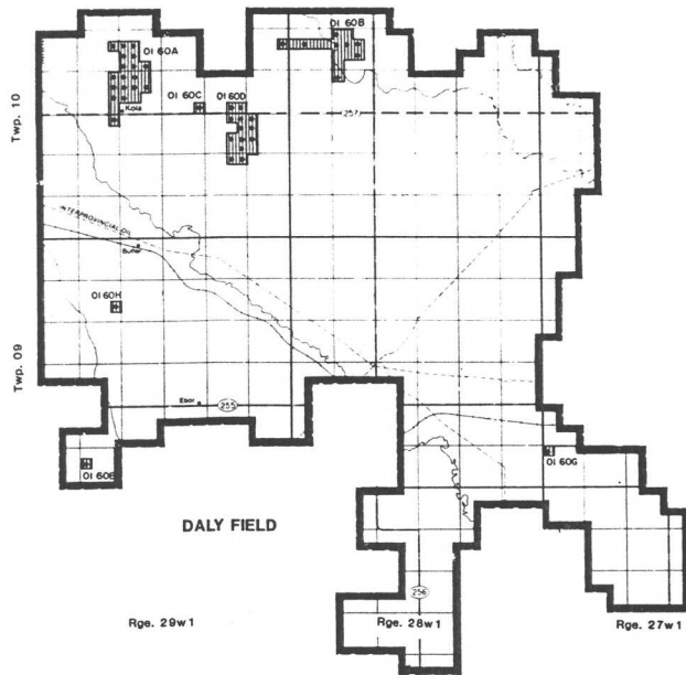
Figure 18: Map showing the producing wells as of January 1991 in Daly field, Manitoba (Martiniuk, 1988).
