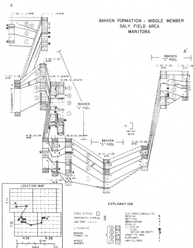
Figure 8: Fence diagram showing the distribution of the lithofacies units of the Middle Member of the Bakken Formation in the Daly field area of Manitoba. Lithofacies represented are described from cores. Sedimentary features, as well as oil staining are indicated.
