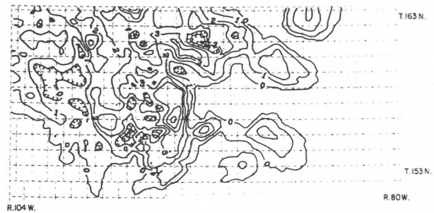
Figure 7: Isopach map showing the distribution of lithofacies unit 3, the producing sandstone, throughout northwestern North Dakota. Contour interval is 1 m (3 ft). Dashed lines are townships and are 10 km (6 mi) on a side.
