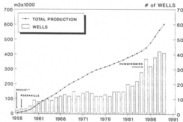
Figure 21: Cumulative production from the Bakken Formation in southeastern Saskatchewan.
