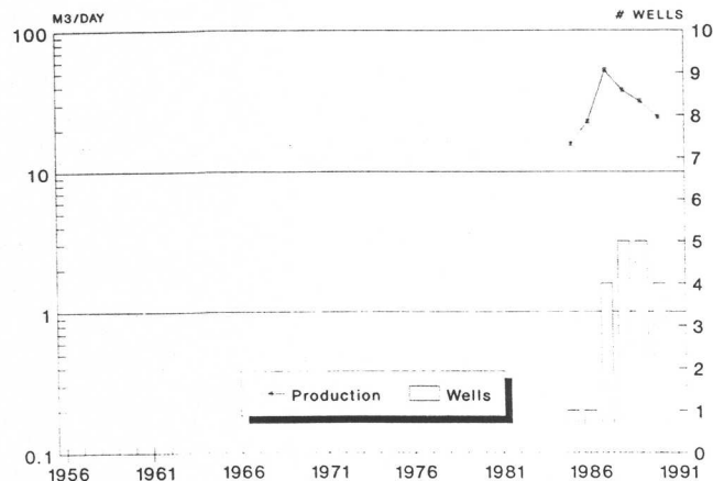
Figure 24: Average daily oil production by year for the Hummingbird Bakken sand pool in Saskatchewan.
