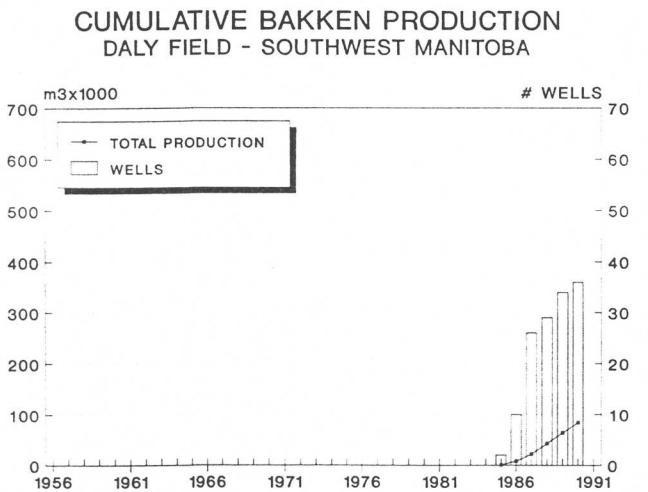
Figure 19: Cumulative production from the Bakken in Daly field in southwestern Manitoba.
