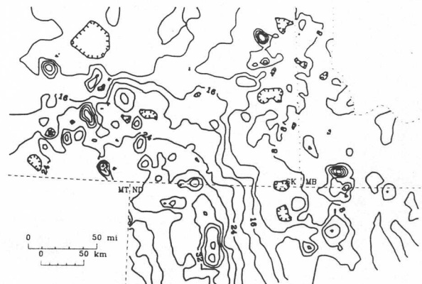
Figure 2: Isopach map of the Bakken Formation for the study area. Contour interval is 4 m (13 ft). Dashed line in northeastern Manitoba is the erosional limit of the Bakken Formation.
