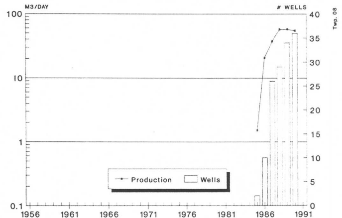
Figure 20: Average daily oil production by year for Daly field in southwestern Manitoba.
